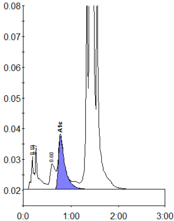
Peak table - ID: 10507923
